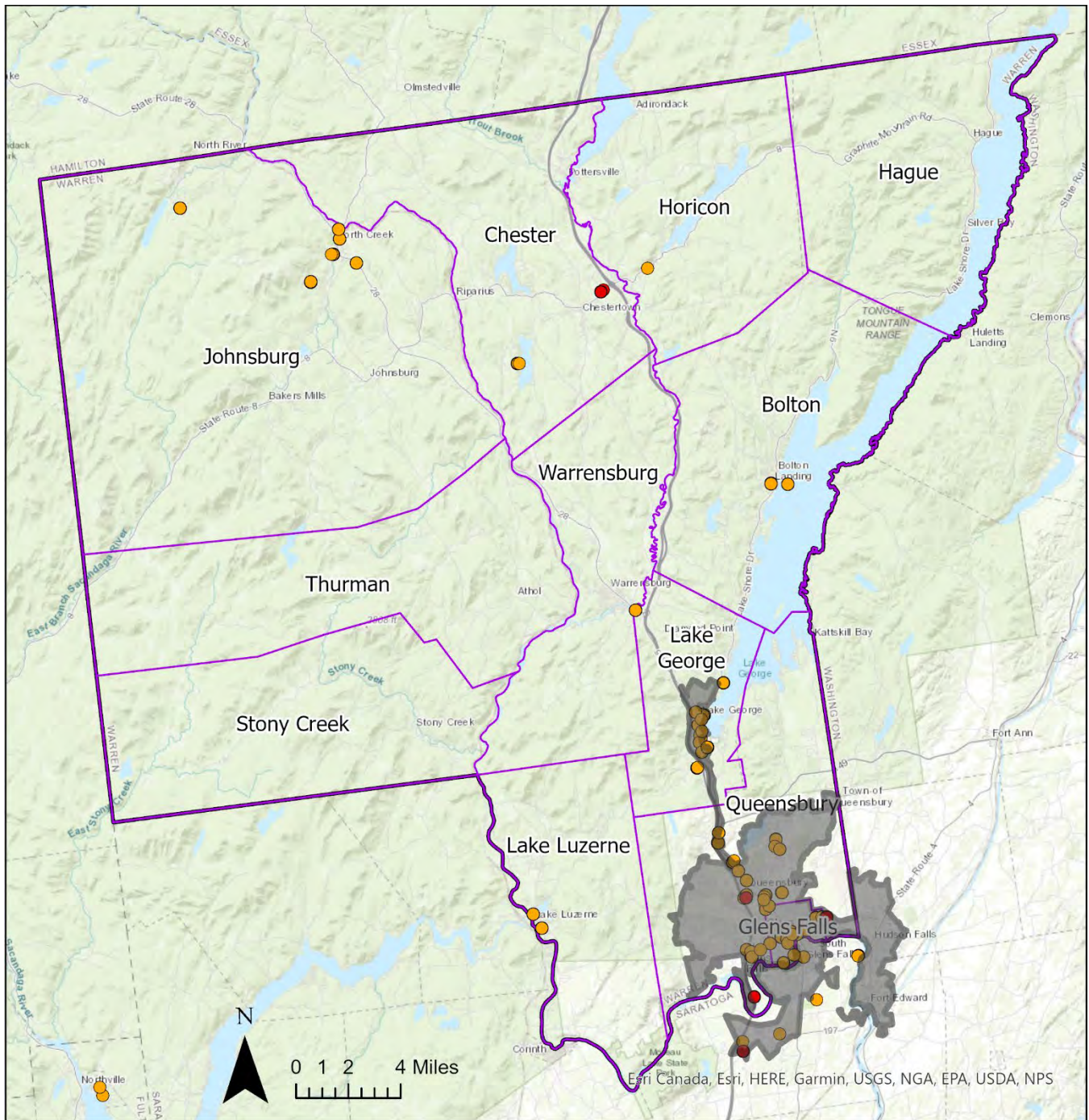
Figure 1 - Context Map
